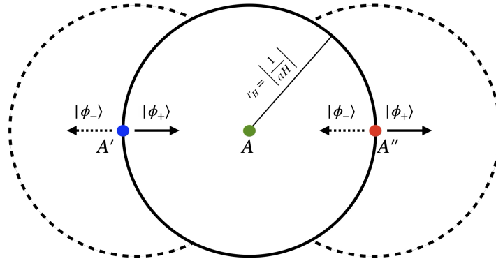
Figure 6. This figure illustrates three comoving (imaginary) observers A, A', A'' with the corresponding comoving horizon radius r_H = \frac{1}{aH} at a moment of dS expansion. We have suppressed here the angular coordinates (\theta, \varphi) . Points A' and A'' are on the horizon of A at antipodal sides of the horizon, that are spacelike separated, i.e., at the angles (\theta, \varphi) and (\pi - \theta, \pi + \varphi) respectively. The dotted circles with the same r_H represent the respective comoving horizons of A' and A'' . In the figure, |\phi_+\rangle, |\phi_-\rangle are defined in (164). In the case of exact dS spacetime, both |\phi\rangle components would give equal two-point correlations at the parity conjugate points (163) due to the \mathcal{PT} symmetric dS vacuum (160). Whereas in the quasi-dS spacetime, we get unequal correlations (180) due to the \mathcal{PT} asymmetric quasi-dS vacuum (175).
